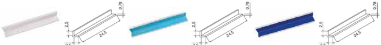
61190 90° Concave Angle (Unglazed)
