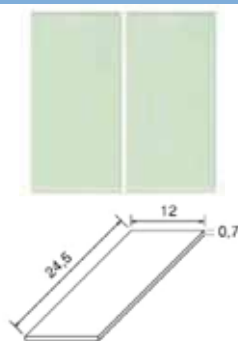
80122.5 Porcelain Tile (Nile Green)
