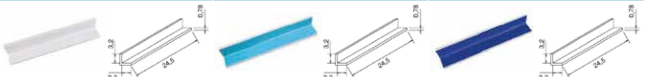
60190 90° Concave Angle (Unglazed)
